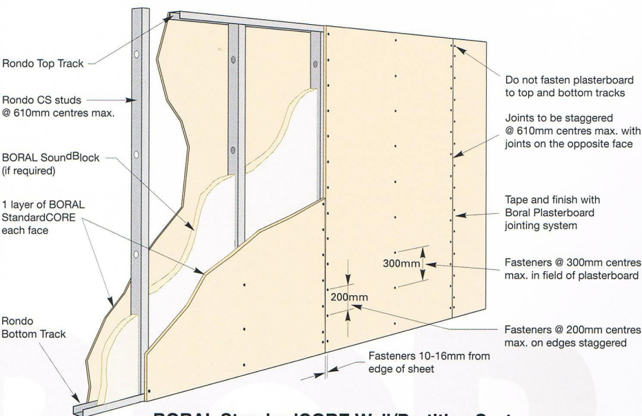
BORAL StandardCORE Wall/Partition System
